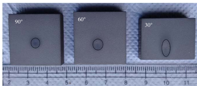
Figure 8. Samples post hot air jet erosion at 90°, 60°, and 30° impact angle.
