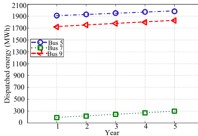
Fig.6. Total dispatched energy for each configuration and over the planning horizon
