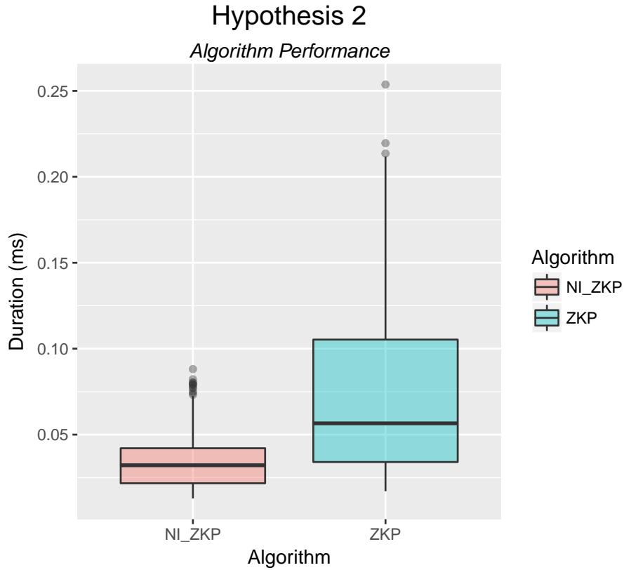
Figure 9: Effect of Authentication Algorithm.
