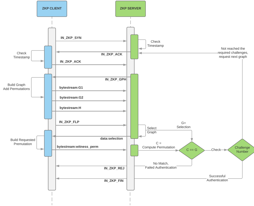
Figure 2: ZKP Client Server Simulation Flow.
