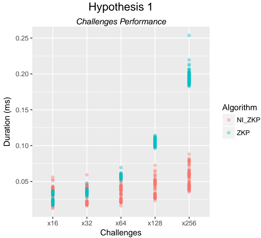
Figure 8: Effect of Authentication Challenges.
