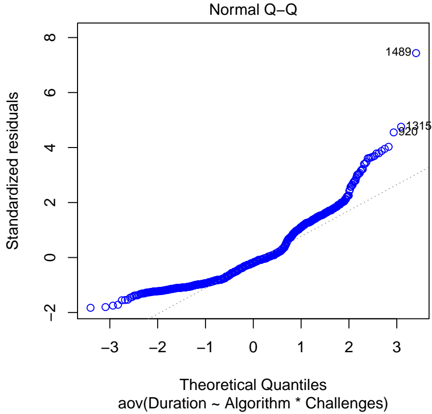
Figure 7: Normal Distribution Plot.
