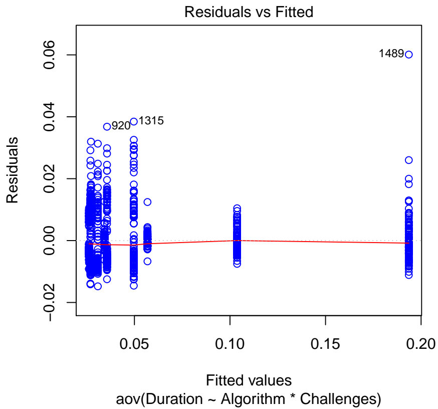
Figure 6: Residuals Vs Fitted Plot.
