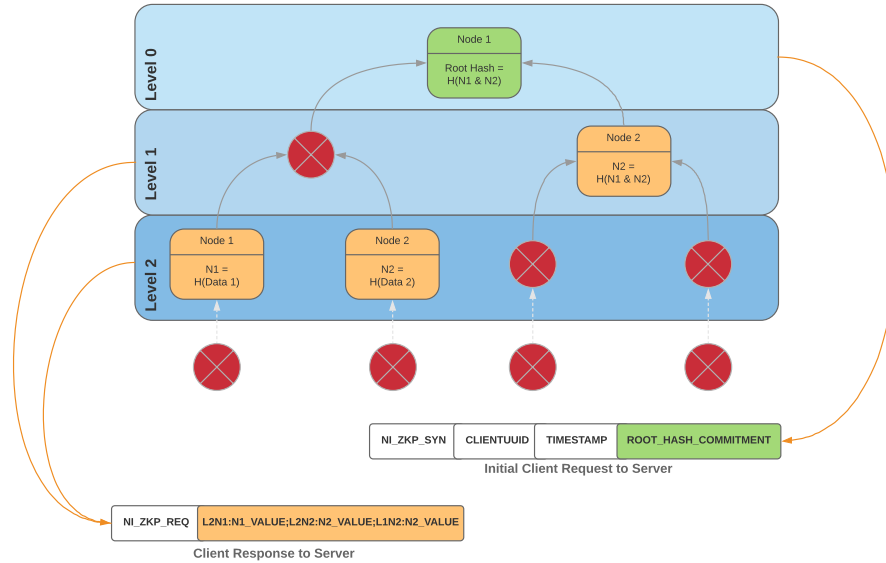
Figure 3: Challenge Packets and Construction of Proof.
