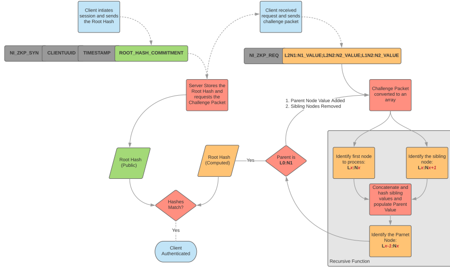
Figure 4: NIZKP Packet Processing.
