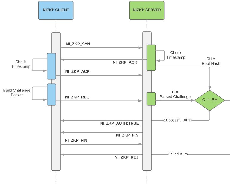
Figure 5: NIZKP Client Server Message Exchange.
