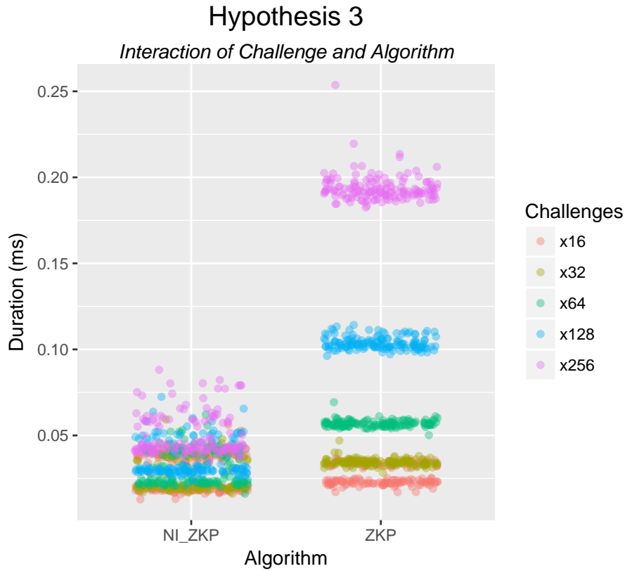
Figure 10: Effect of Interaction of Algorithm and Challenges.
