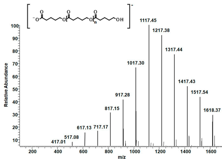
Figure 7. ESI-MS n spectrum (negative ion mode) of poly( \delta -valerolactone) precursor ion at m/z 917 and the respective parent ions with different chain length (MS 2 –MS 9 ), (Sample 1, Table 1).
