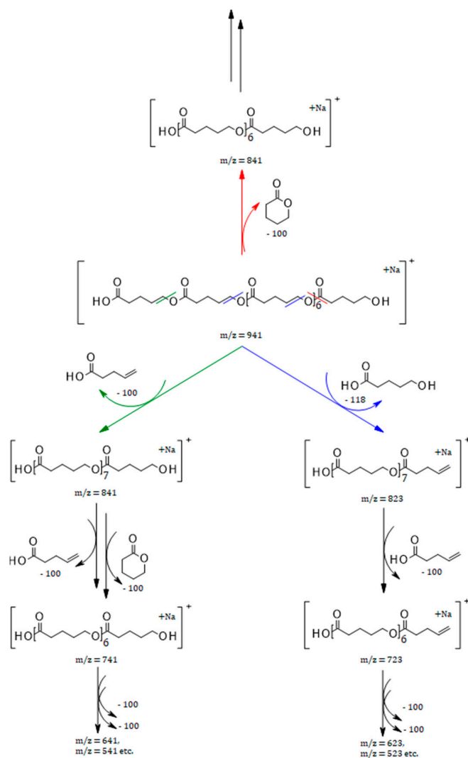
Scheme 3. Possible fragmentation pathways for sodium adducts of benzyl- and hydroxy-terminated PVL oligomers at m/z 941.
