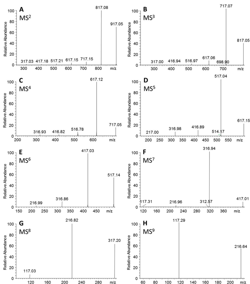
Figure 8. ESI-MS n spectra (negative ion mode) of poly( \delta -valerolactone) precursor ion at m/z 917 and the respective parent ions with different chain length (MS 2 (A)–MS 9 (H)), (Sample 1, Table 1).
