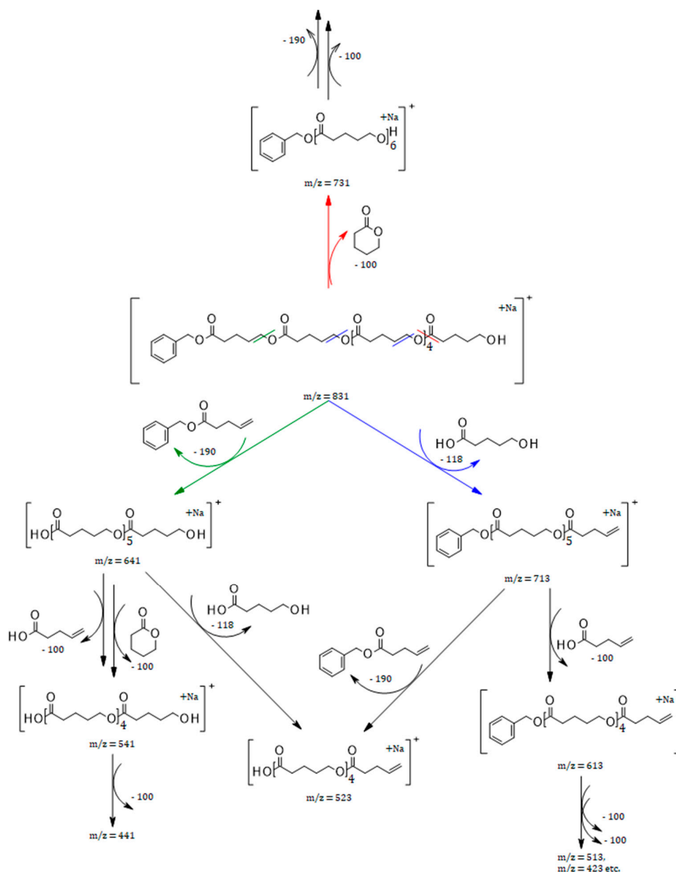
Scheme 2. Possible fragmentation pathways for sodium adducts of benzyl- and hydroxy-terminated PVL oligomers at m/z 831.
