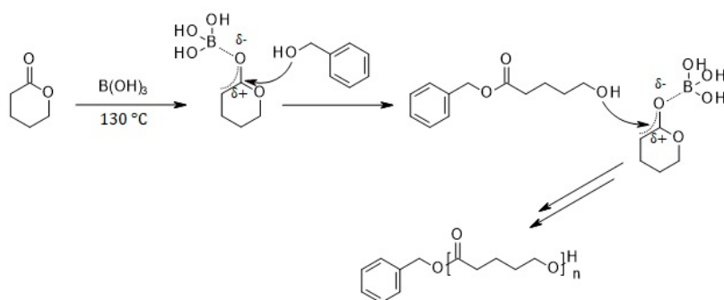
Scheme 1. The ring-opening polymerization of \delta -valerolactone initiated by benzyl alcohol with the presence of boric acid as a catalyst to activate the monomer.
