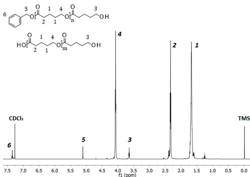
Figure 1. Proton nuclear magnetic resonance ( 1 H-NMR) spectrum of poly(δ-valerolactone) oligomers (Sample 1, Table 1).
