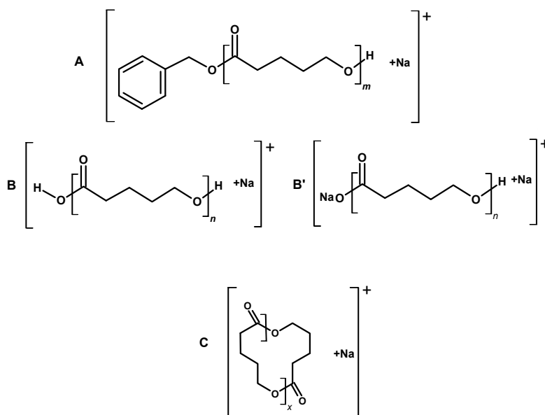
Figure 3. The structures of the ions observed in ESI-MS of PVL.
