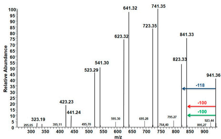
Figure 5. ESI-MS/MS spectrum of the sodium adducts poly( \delta -valerolactone) oligomers with hydroxyl and carboxyl end groups at m/z 941 (Sample 1, Table 1).
