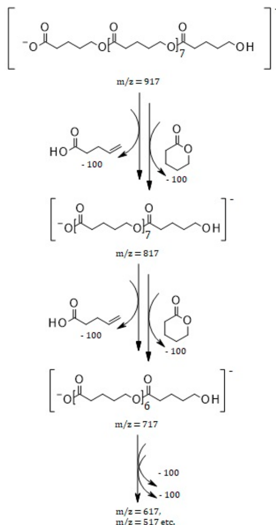
Scheme 4. Possible fragmentation pathways of the anion of PVL oligomers terminated by hydroxyl and carboxylic end group.
