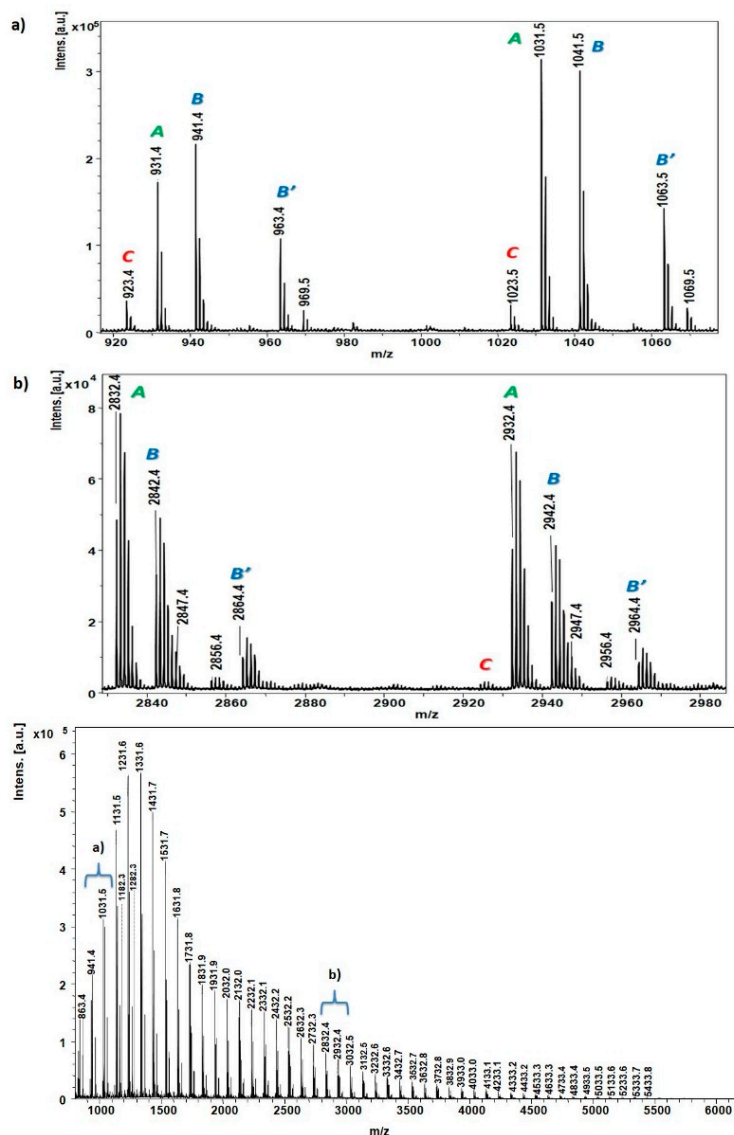
Figure 6. MALDI-TOF-MS spectrum (positive ion mode) of poly( \delta -valerolactone) together with two spectral expansions in the mass range: (a) m/z 910–1100 and (b) m/z 2810–3090 (Sample 2, Table 1).
