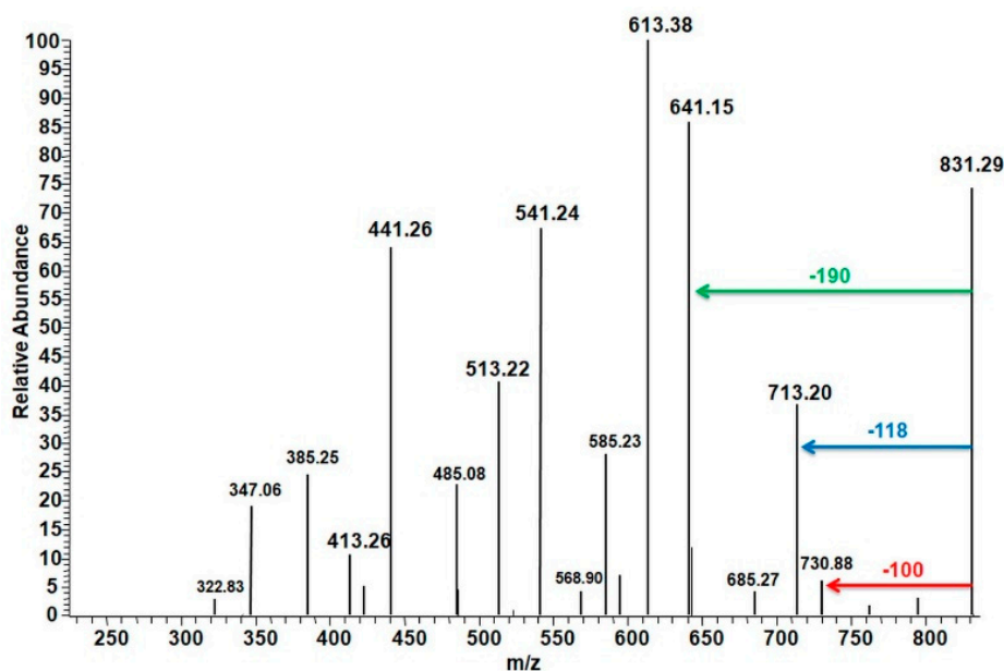
Figure 4. ESI-MS/MS spectrum of the sodium adducts of poly( \delta -valerolactone) oligomers with benzyl and carboxyl end groups at m/z 831 (Sample 1, Table 1).
