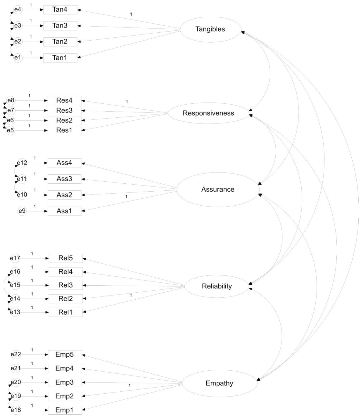
Figure 1. First-order measurement model.
