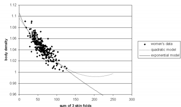
Figure 4. The quadratic model and proposed alternative exponential power-function model for women.
