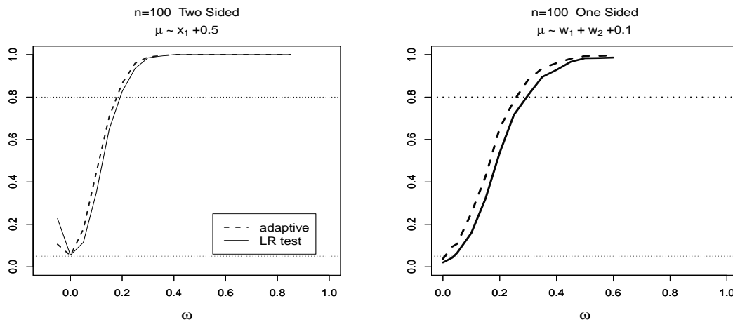
Figure 7: Power under hybrid estimator (covariate model, left: alternative H_1^{(a)} ; right: H_1^{(b)} )
