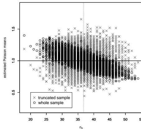
Figure 1: Estimation from the zero-truncated and whole sample
