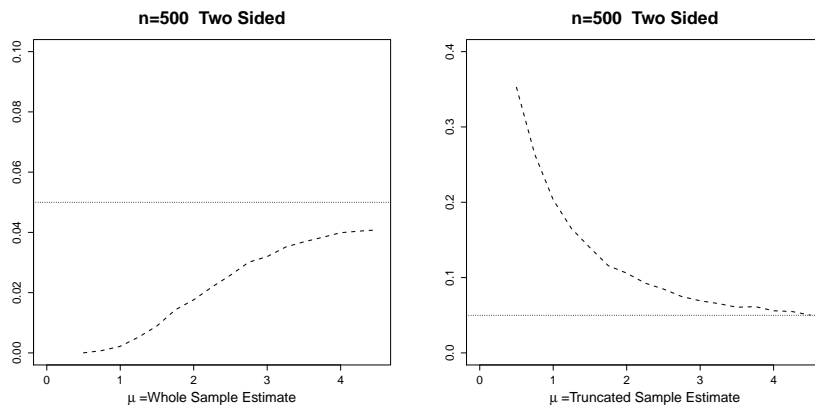
Figure 2: Attainment rate using \hat{\mu}_W and \hat{\mu}_T
