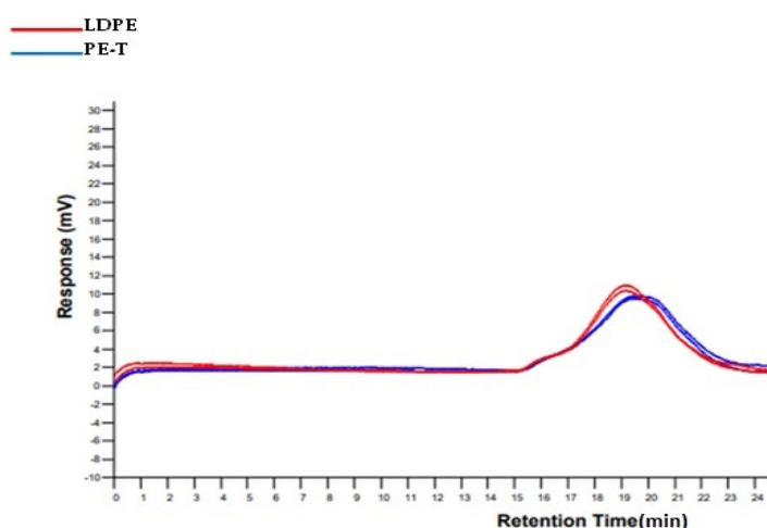
Figure 4. The GPC refractive index chromatograms for duplicate runs of PE-T and plain LDPE.
