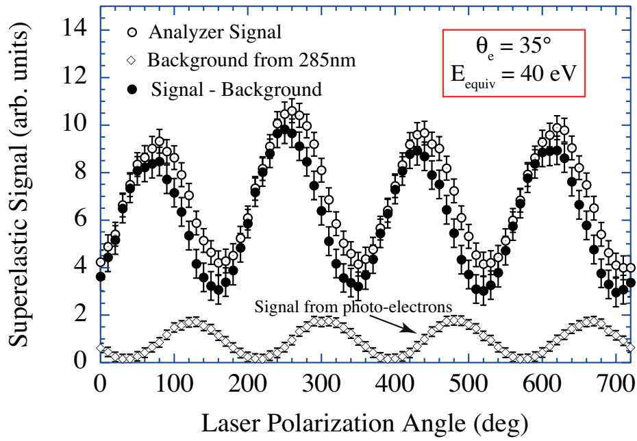
FIG 5. Signal from the analyzer when the laser-beam was on-resonance with the atomic beam, as the half wave-plate was rotated through 360^\circ . The ‘raw’ superelastic signal is shown as open circles. The lower signal (shown as diamonds) was measured by adjusting the gun energy by 3 eV, so that there was no contribution from superelastic scattering. This signal arises from photoelectrons produced by fluorescence radiation striking surfaces inside the analyzer. The closed circles show the resulting superelastic signal when this background was subtracted from the raw signal.
