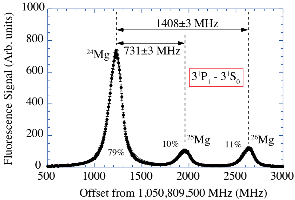
FIG 3. Fluorescence excitation spectra observed using the UV photodiode, showing excitation of the different isotopes of magnesium by the laser beam. The spectrum is offset from 1050,809,500 MHz so that a comparison of the isotopic mass-shifts in energy can be seen. The dominance of the ^{24}\text{Mg} isotope is clearly observed. These isotopes were selected for the superelastic studies discussed in this paper.
