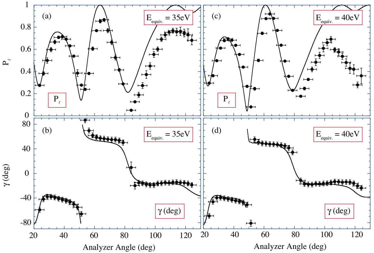
FIG 6. Measurement of the (P_\ell, \gamma) parameters for electron-impact excitation of the ground state of Mg to 3^1P_1 using the superelastic technique for equivalent incident energies of 35 eV and 40 eV, compared to theoretical calculations using the CCC model with 513 target states (solid line).
