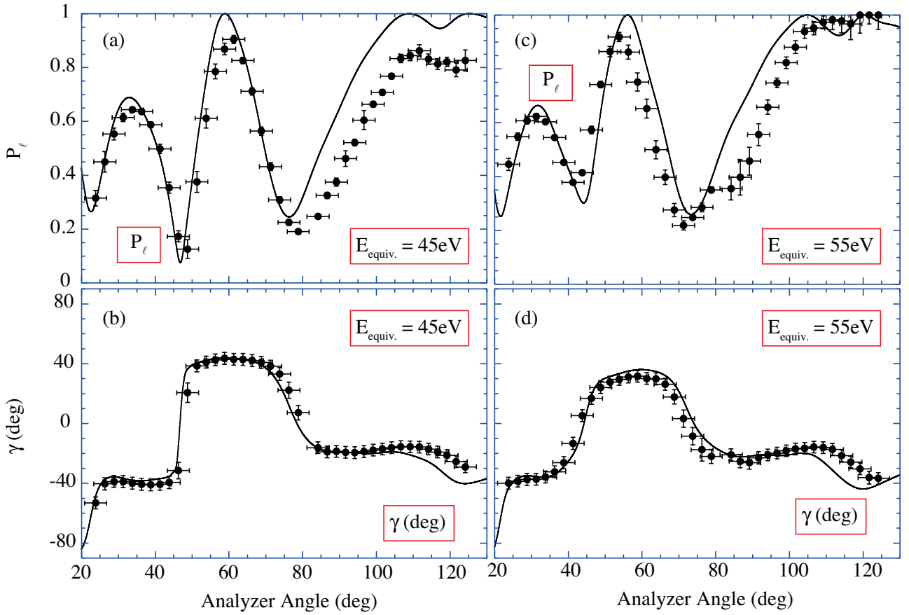
FIG 7. Same as for Fig.6, except for equivalent incident energies of 45 eV and 55 eV.
