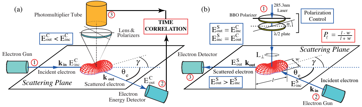
FIG 1. Determining the charge-cloud alignment and orientation following a collision. (a) In coincidence studies, the incident electron (1) excites the target and is scattered through an angle \theta_e to the detector (2). Photons emitted from relaxation of the atom are then detected (3) for different polarizations of the radiation. The scattered electron and correlated photon are then detected in coincidence. (b) In superelastic scattering studies the arrow of time is reversed, so that the state is initially excited by polarized laser radiation (1). An incident electron (2) then de-excites the target, the scattered superelastic electrons being detected as a function of laser polarization (3). Alignment of the charge cloud is determined through the parameters P_\ell and \gamma , and the angular momentum transferred during the collision is given by L_\perp .
