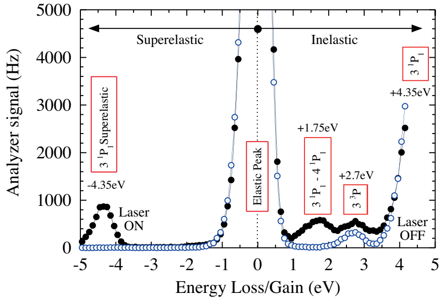
FIG 4. Energy loss/gain spectrum from electron interaction with ^{24}\text{Mg} atoms in the interaction region, referenced to the position of the elastic peak.
