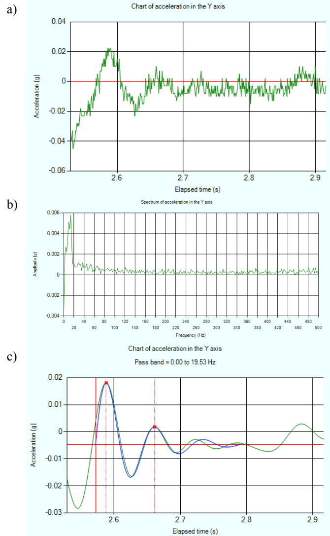
Figure 1: Acceleration-time data before filtering (a), Fourier transform of data (b) and acceleration-time data after filtering (c).
