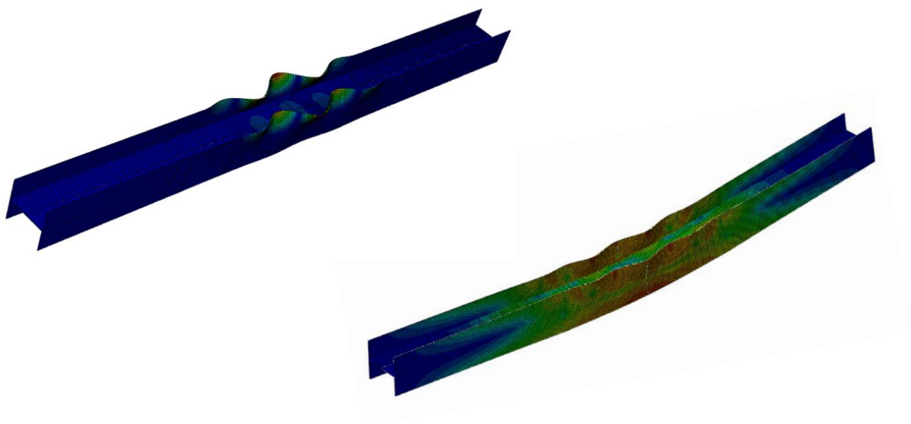
a) I-sections
