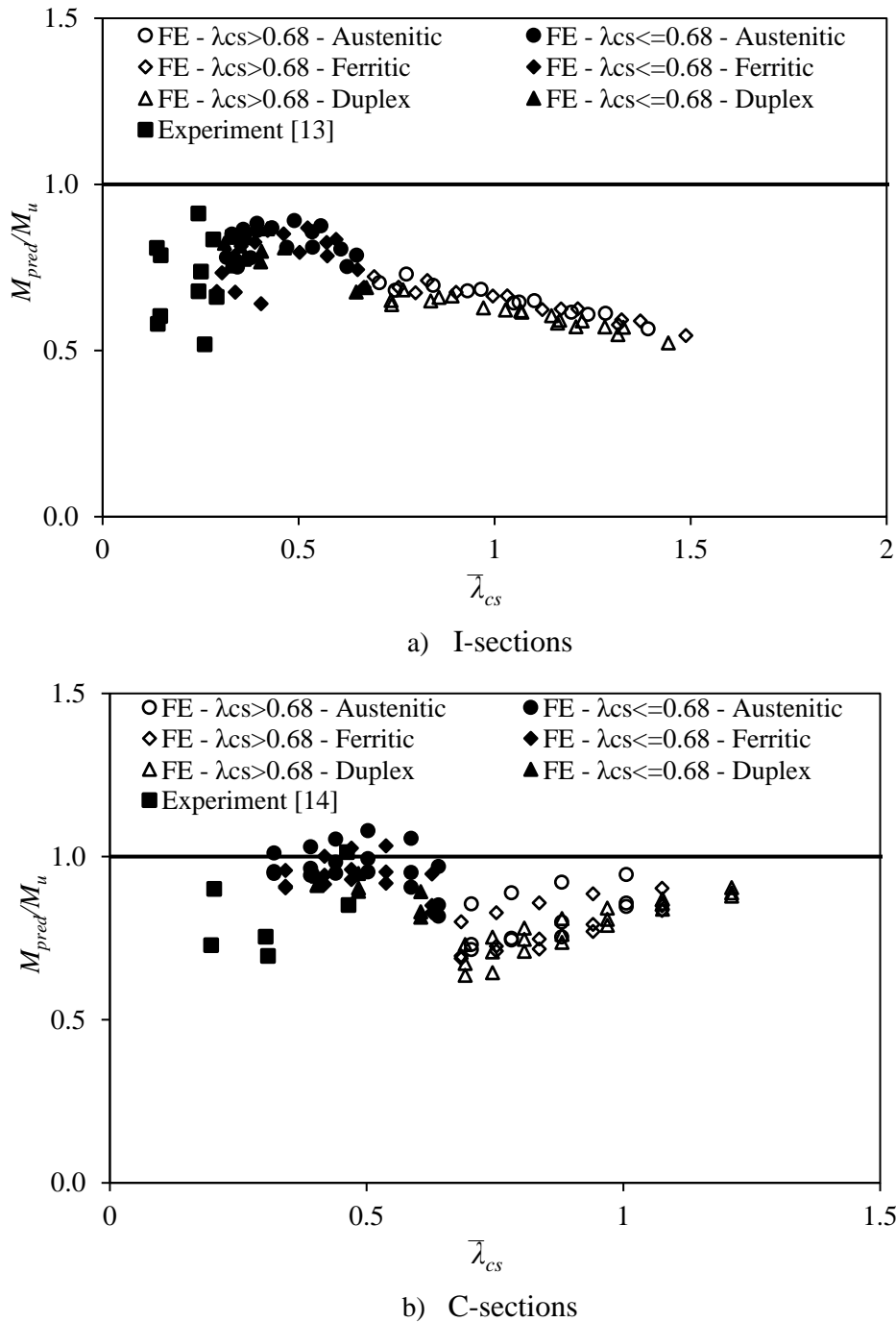
Figure 11: Assessment of the Continuous Strength Method.
