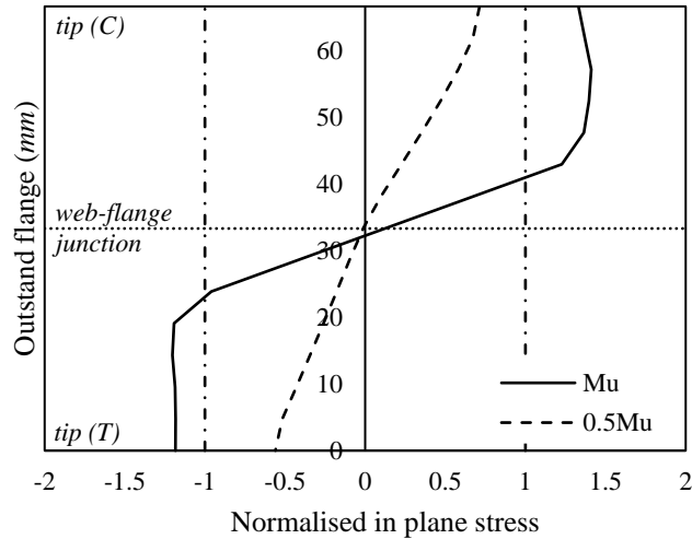
c) Duplex (100×66.67×1.33 - h/b=1.5 , c_f/(t_f\epsilon)=37.7 , \lambda_{cs}=1.33 )
