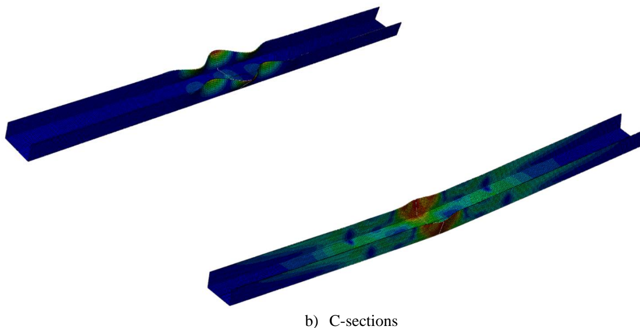
Figure 7: Typical elastic buckling (top) and nonlinear (bottom) failure modes from parametric study.
