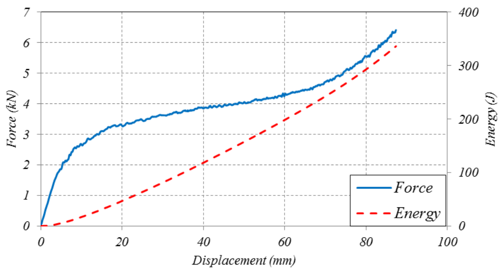
Fig. 11. Force and energy responses of the STFIIIC system.
