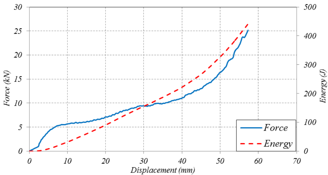
Fig. 14. Force and energy responses of the STFISC system.
