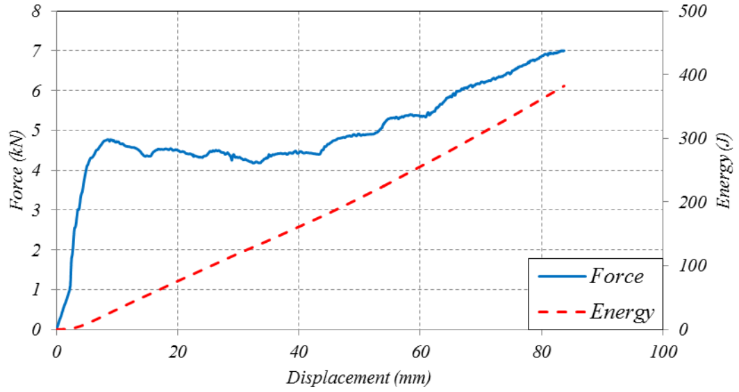
Fig. 29. Force and energy responses of the STCICC system.
