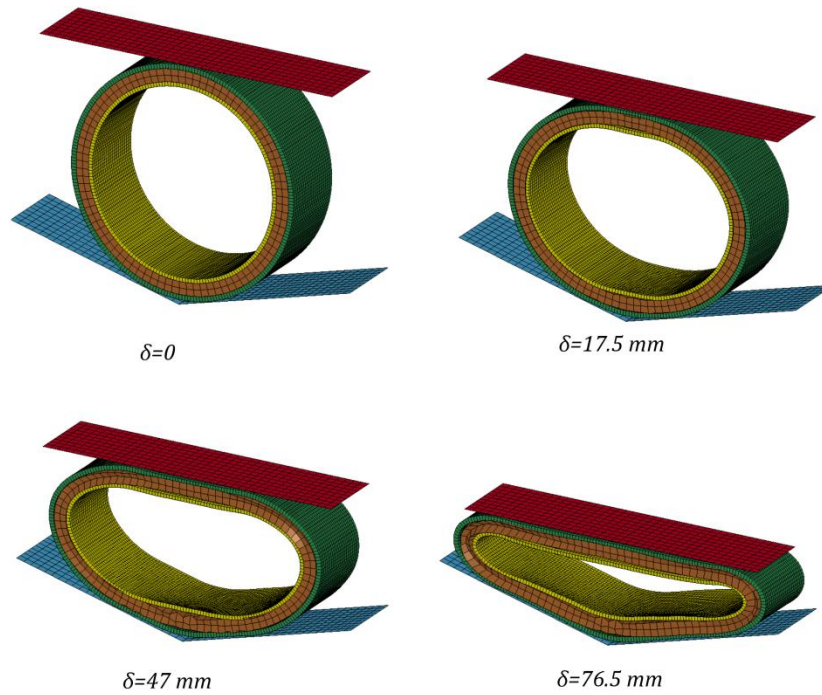
Fig. 13. Collapse sequence of the STFIC under quasi-static loading.
