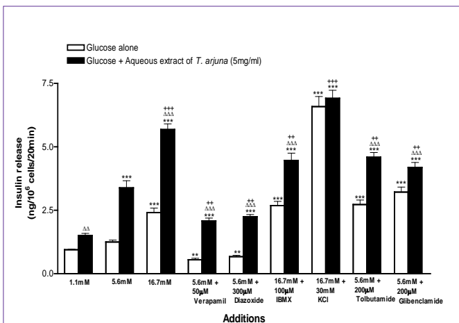
Figure 2: Modulation of Terminalia arjuna extract-induced insulin secretion by established stimulators and inhibitors of beta cell function. Values are mean ± SEM of 8 separate observations. **P<0.01, ***P<0.001 compared to glucose (control) in presence or absence of plant extract. ΔΔP<0.01, ΔΔΔP<0.001 compared to the respective incubations in absence of plant extract. **P<0.01, ***P<0.001 compared to 16.7mM glucose in presence or absence of plant extract.
