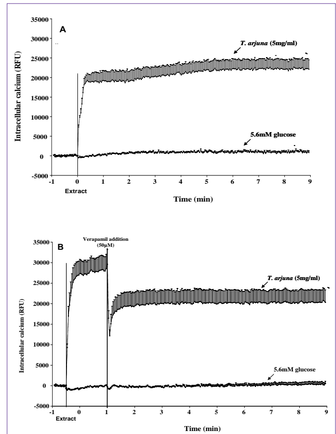
Figure 4: Effects of Terminalia arjuna on intracellular Ca 2+ influx in the absence (A) and presence of Verapamil (B). Intracellular calcium concentration were measured by fluorescence spectroscopy in BRIN-BD11 cells incubated with KRB buffer containing FLIPR calcium dye and 5.6mM glucose in the presence or absence of plant material (5mg/ml) (Figure 4A). Verapamil (50µM) was added 60 seconds after the commencement of the experiment in Figure 4B. Data was collected every 1.25 seconds over a period of 540 seconds. Values are mean ± SEM of 6 separate observations.
