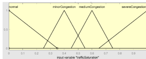
Figure 4. Membership function for traffic saturation
