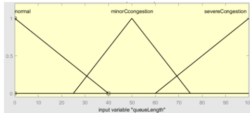
Figure 5. Membership function for queue length
