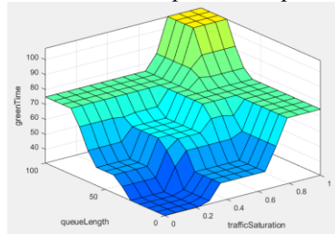
Figure 8. Correlation between Inputs (queue length and traffic saturation) and Output Fuzzy Variables
