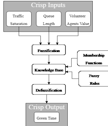
Figure 3. Computation of output Green Time
