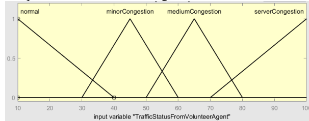
Figure 6. Membership function for traffic status from volunteer agent
