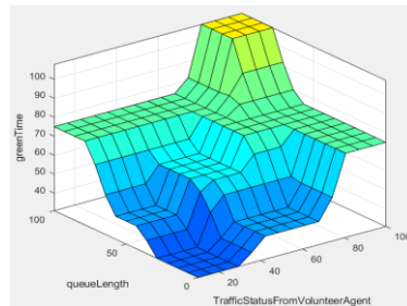
Figure 10. Correlation between Inputs (queue length and traffic status from volunteer agent) and Output Fuzzy Variables
