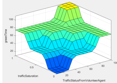
Figure 9. Correlation between Inputs (traffic saturation and traffic status from volunteer agent) and Output Fuzzy Variables
