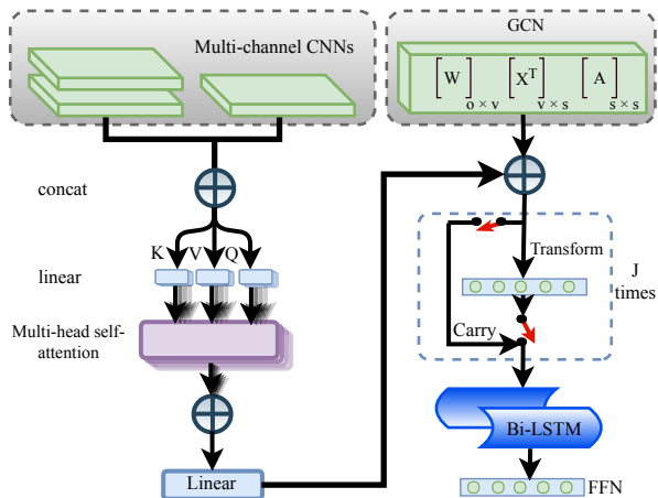
Figure 1: A hybrid sequence labeling approach integrating GCN (o: output dimension; v: word vectors dimension; s: sentence length) and Self-Attention.
